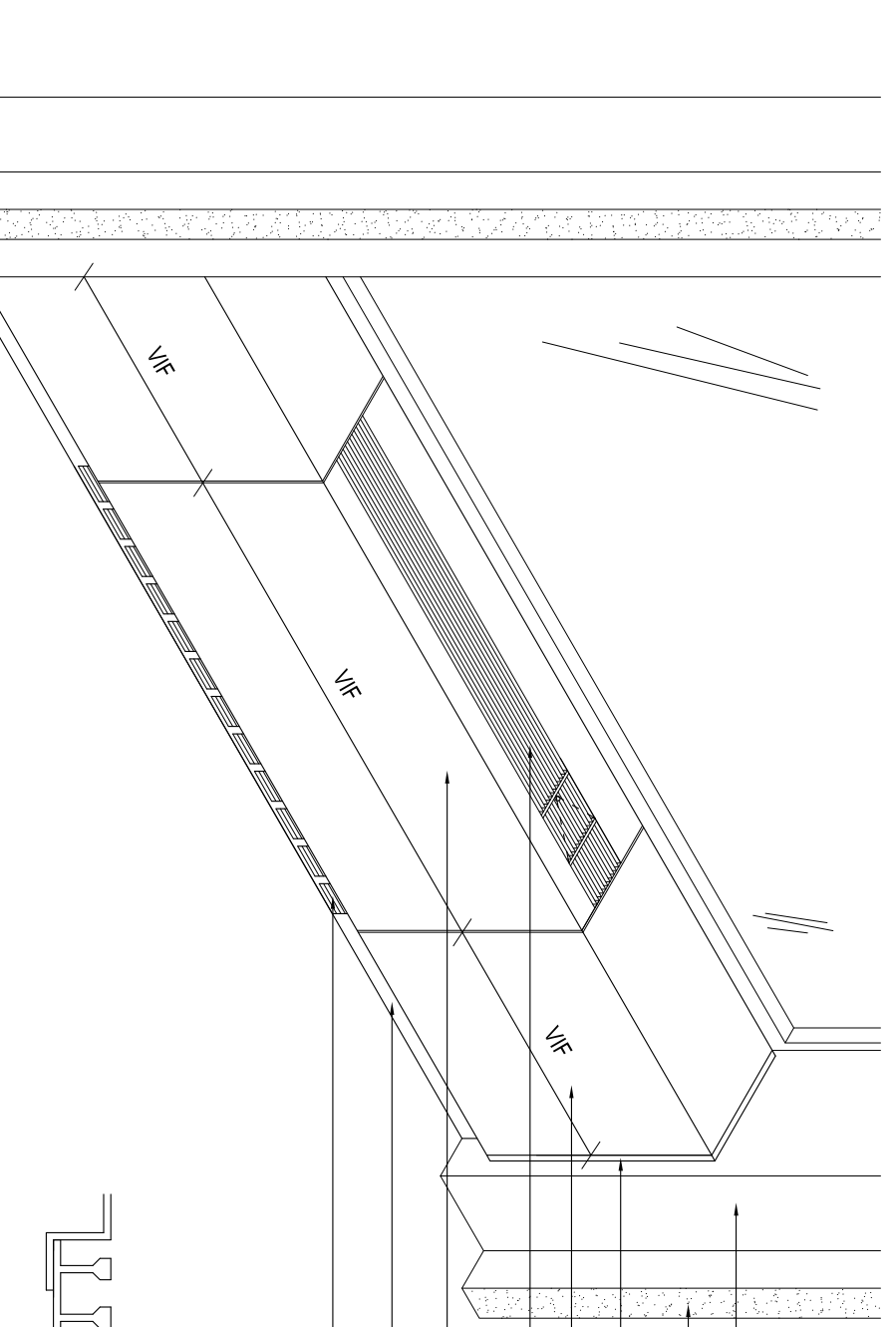
SECTION @ GRILLE
